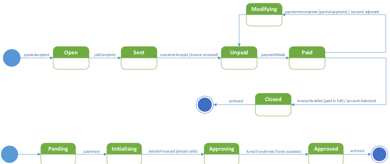
State Machine Diagram: Invoice (top), Payment (bottom)
